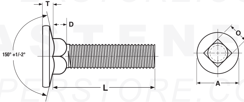
FLAT HEAD CARRIAGE BOLTS, SQUARE NECK
