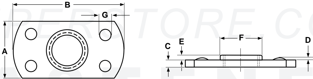
TAB WELD NUTS - CENTER HOLE DESIGN WITH MULTIPLE PROJECTIONS
