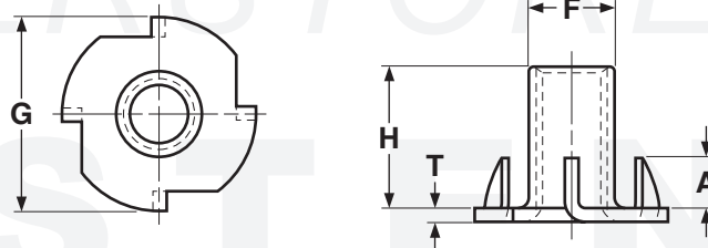
4-PRONG
