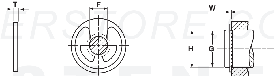
TYPE E RETAINING RINGS
