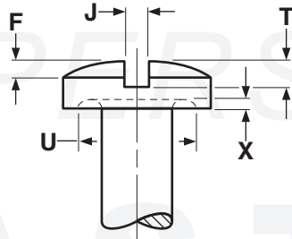
SLOTTED BINDING HEADS UNDERCUT FOR MACHINE SCREWS
