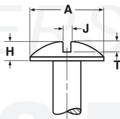
TRUSS HEADS FOR MACHINE SCREWS
