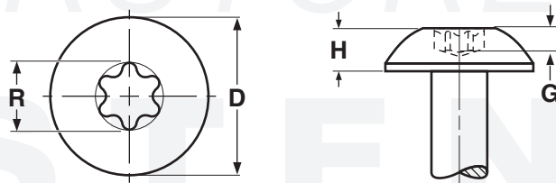
SIX-LOBE TRUSS HEADS
