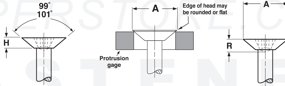
PHILLIPS UNDERCUT 100° FLAT HEADS FOR MACHINE SCREWS
