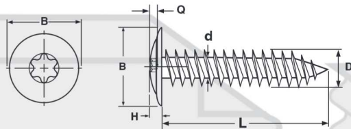
Six-Lobe Recess
