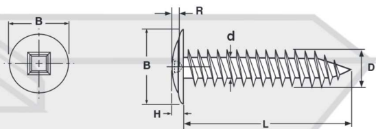
Square Recess
