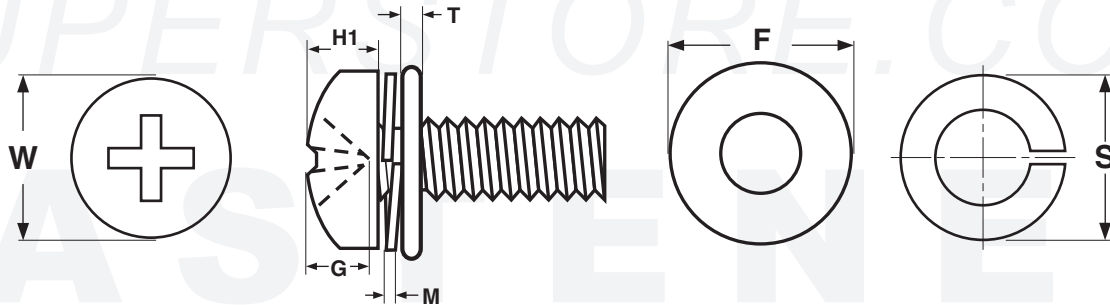
PAN PHILLIPS DOUBLE WASHER SEMS (SPLIT-LOCK & REGULAR FLAT WASHERS)
