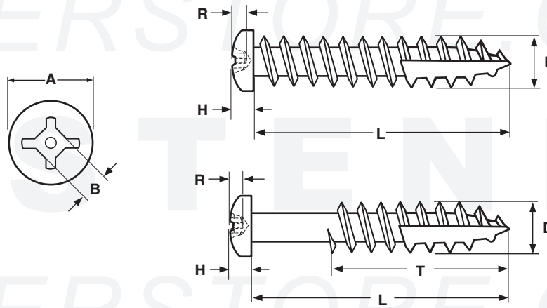
PAN SQUARE-PHILLIPS RECESS DEEP THREAD WOOD SCREW WITH TYPE-17 POINT
