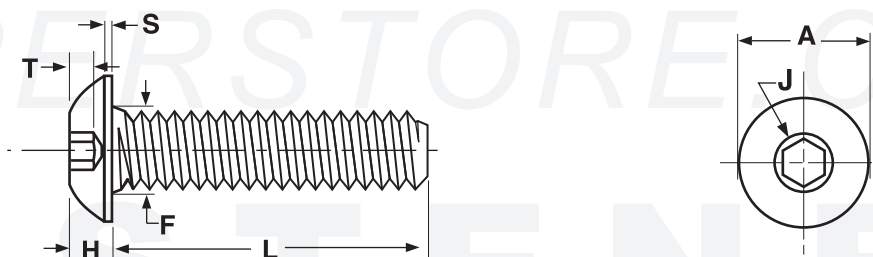
SOCKET BUTTON HEAD CAP SCREWS - ALLOY STEEL
